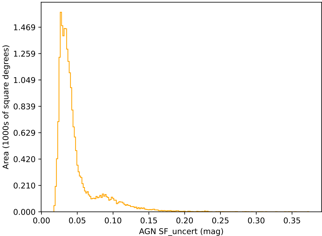
roll_uniform_early_half_mjdp67_v3.4_10yrs r band: AGN SF_uncert
