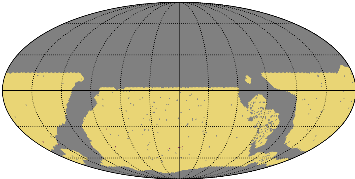
roll_uniform_early_half_mjdp67_v3.4_10yrs WFD: RapidRevisits
