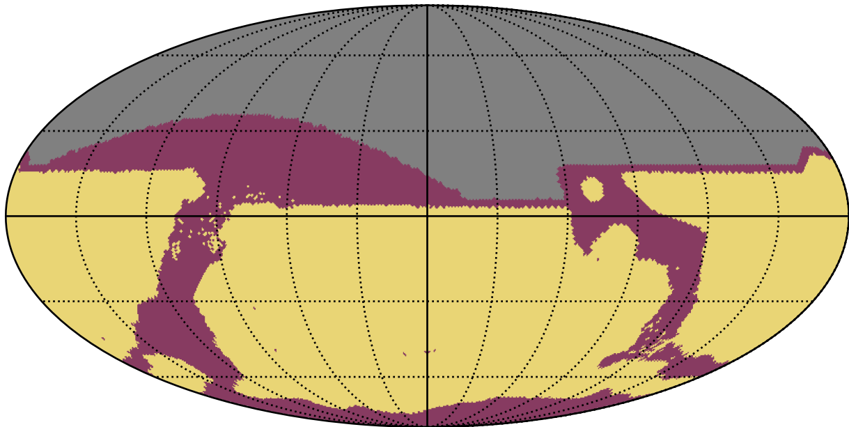
roll_uniform_early_half_mjdp67_v3.4_10yrs All sky: RapidRevisits
