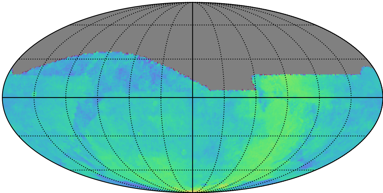
roll_uniform_early_half_mjdp67_v3.4_10yrs All sky: Parallax Coverage @ 24.0
