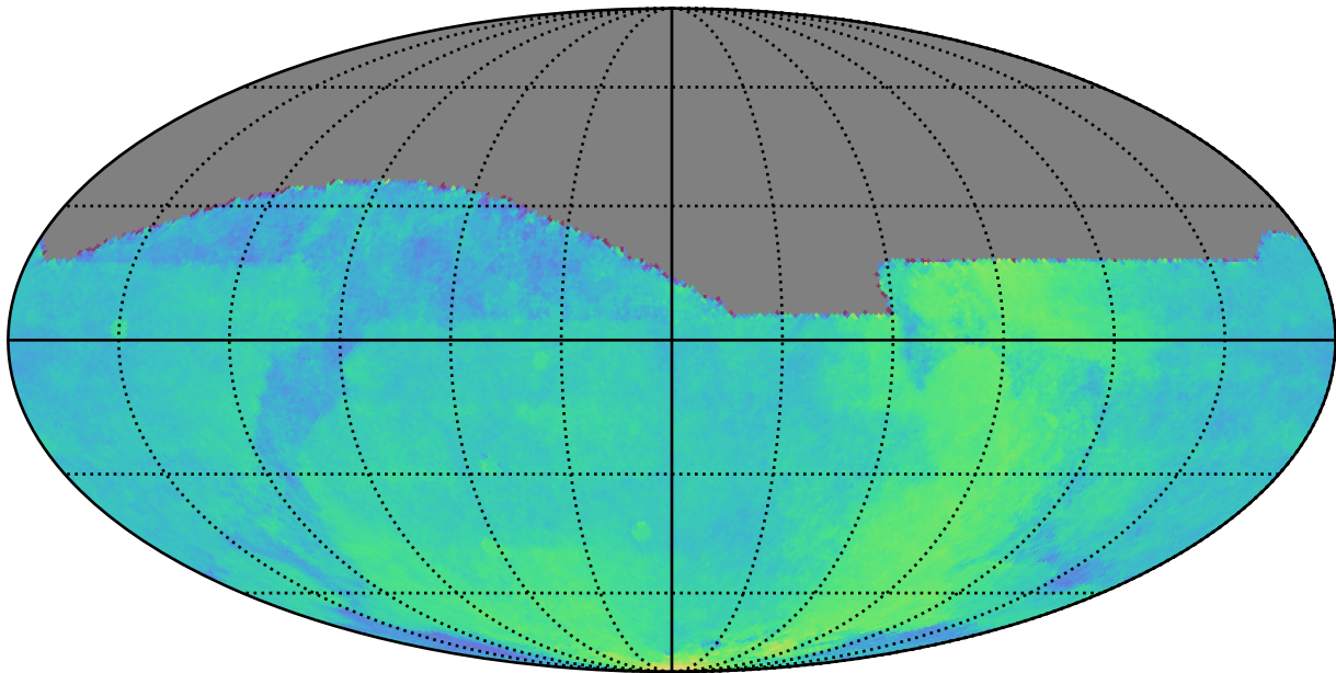
roll_uniform_early_half_mjdp67_v3.4_10yrs All sky: Parallax Coverage @ 22.4
