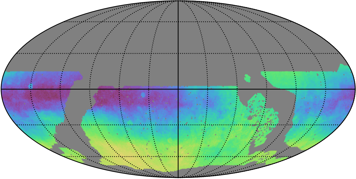
roll_uniform_early_half_mjdp67_v3.4_10yrs WFD: Parallax-DCR degeneracy @ 24.0
