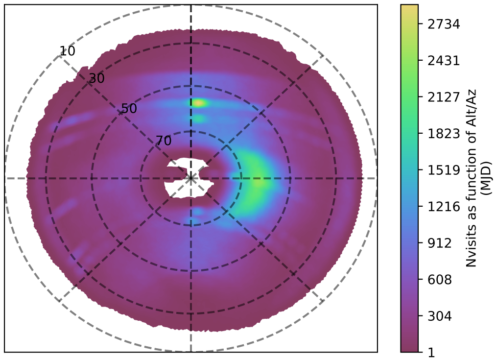
roll_uniform_early_half_mjdp67_v3.4_10yrs i band: Nvisits as function of Alt/Az
