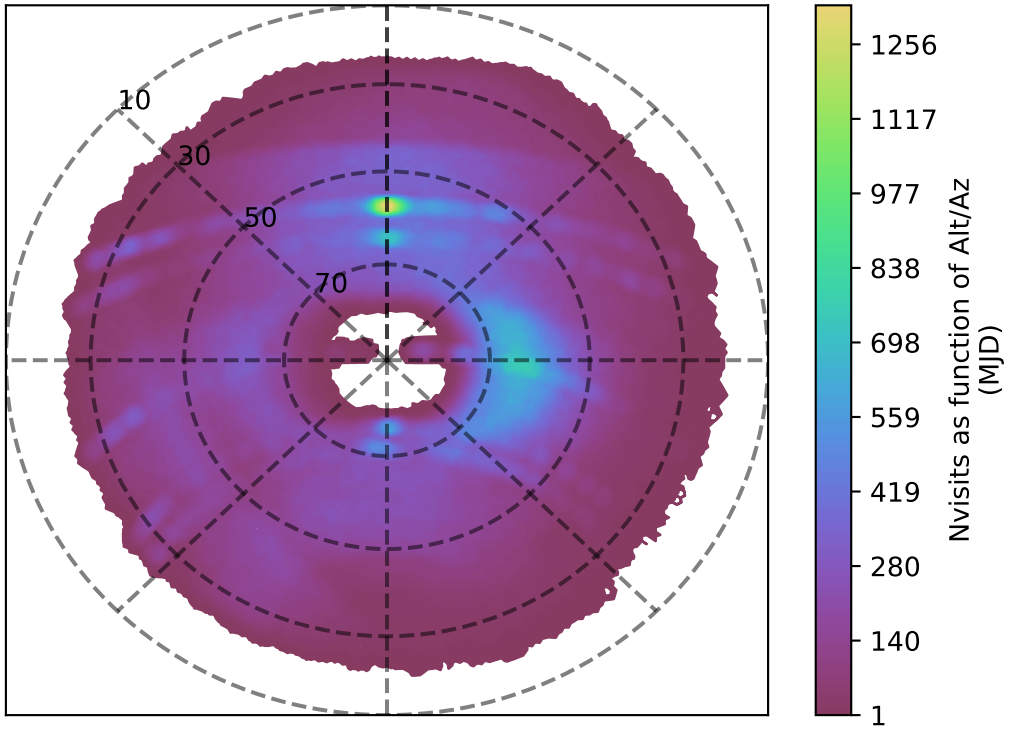
roll_uniform_early_half_mjdp67_v3.4_10yrs g band: Nvisits as function of Alt/Az
