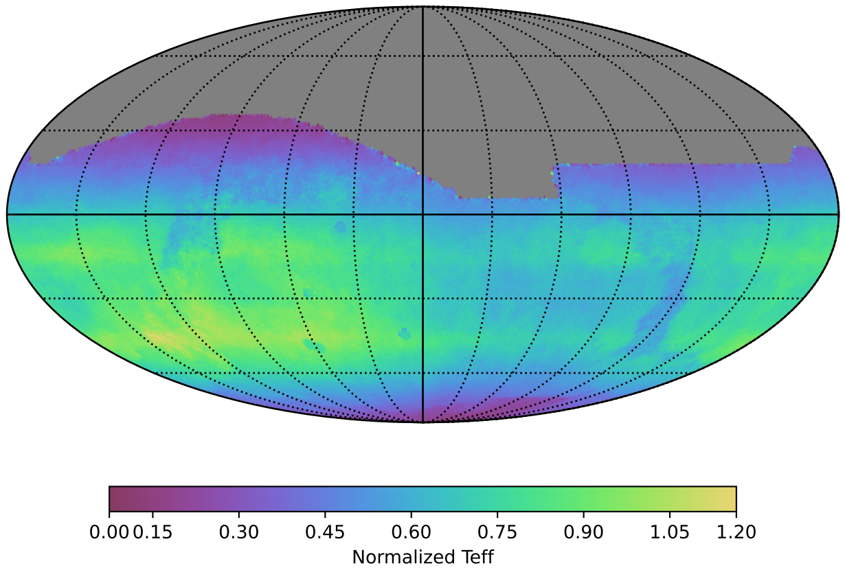
roll_uniform_early_half_mjdp67_v3.4_10yrs All sky all bands: Normalized Teff
