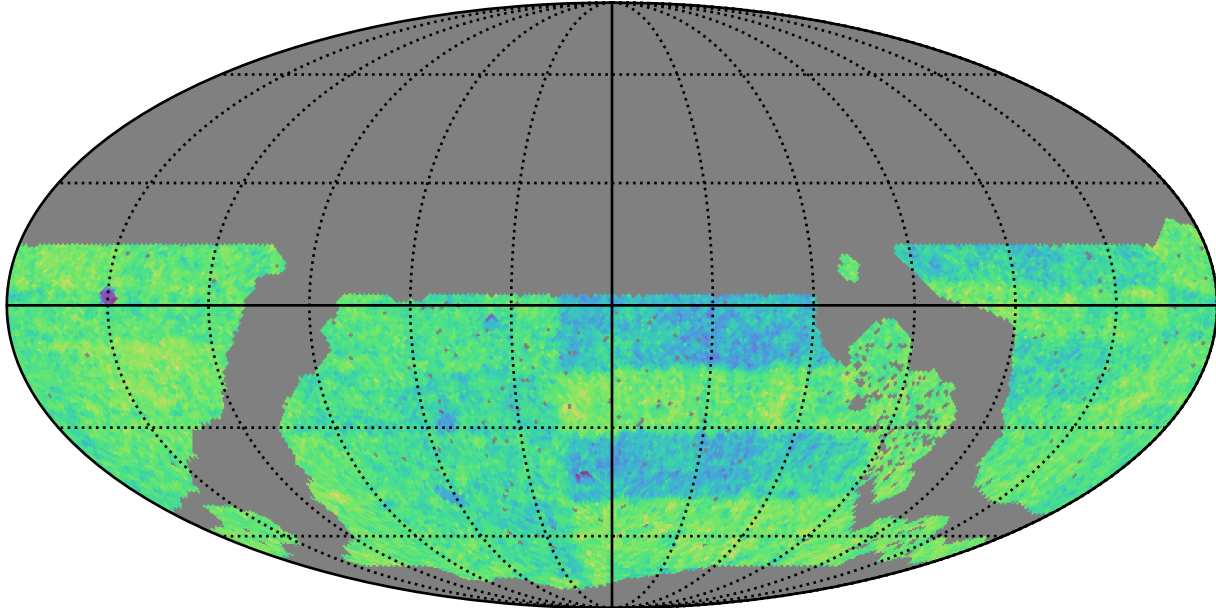
roll_uniform_early_half_mjdp67_v3.4_10yrs WFD: Normalized Proper Motion Uncert @ 20.5
