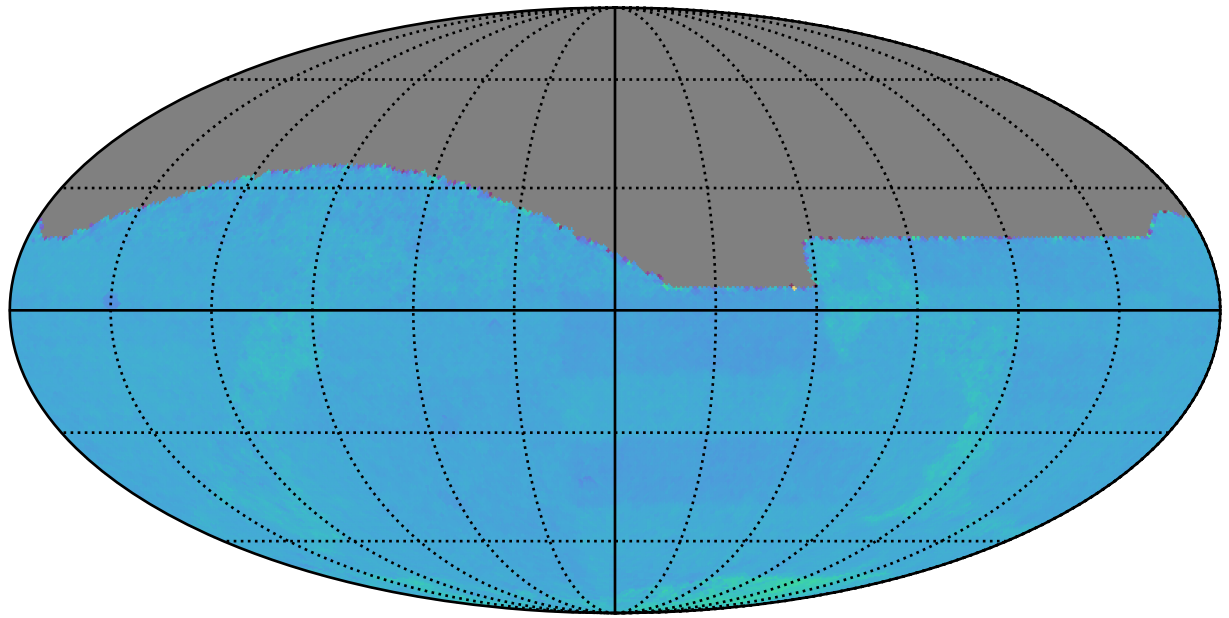
roll_uniform_early_half_mjdp67_v3.4_10yrs All sky: Normalized Proper Motion Uncert @ 20.5
