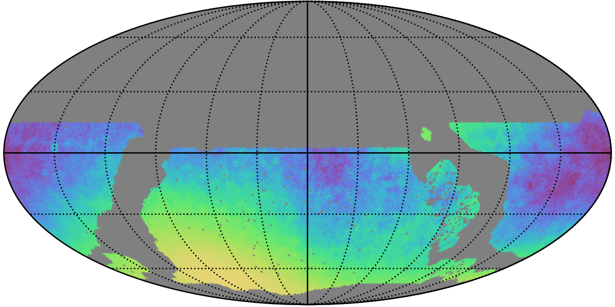
roll_uniform_early_half_mjdp67_v3.4_10yrs WFD y band only: Normalized Parallax Uncert @ 21.3
