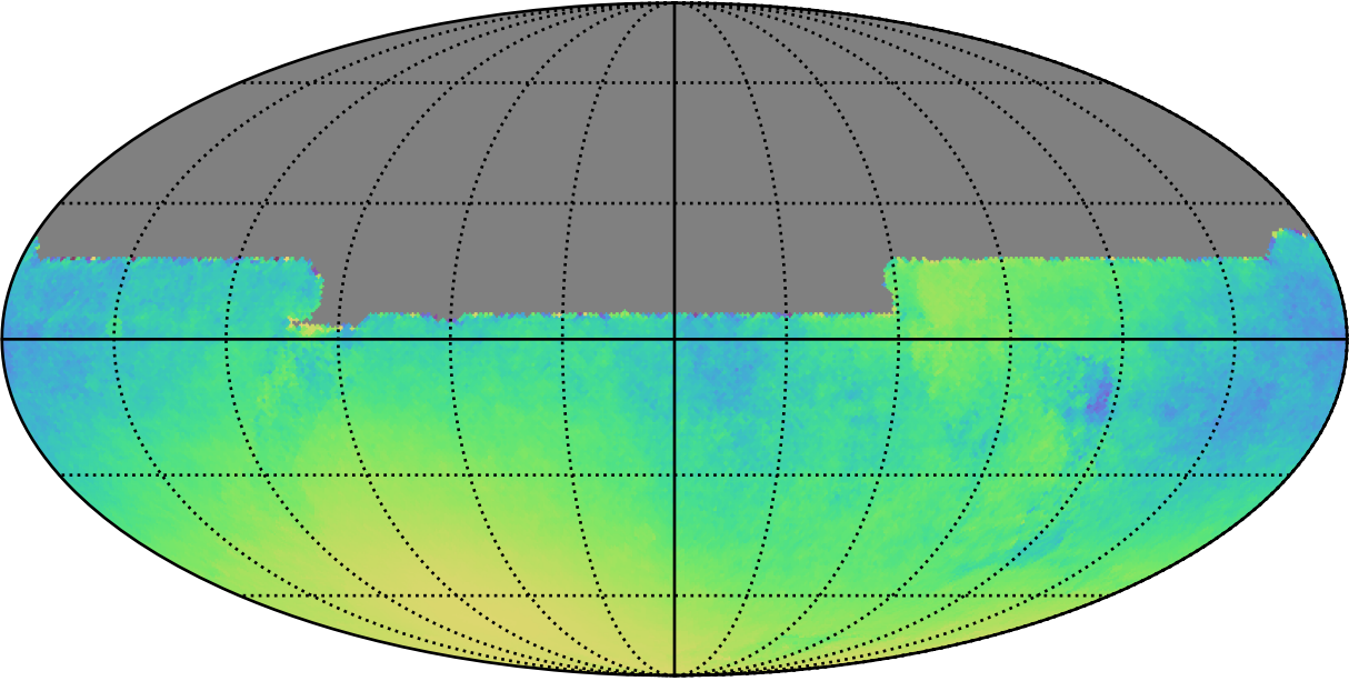
roll_uniform_early_half_mjdp67_v3.4_10yrs All sky y band only: Normalized Parallax Uncert @ 21.3
