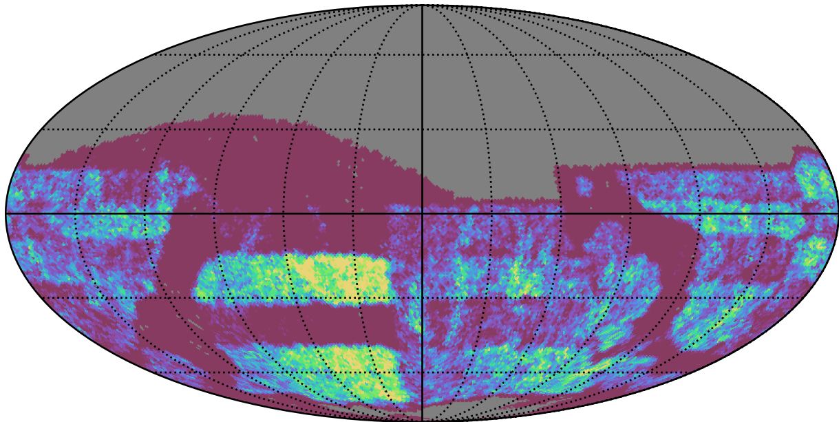
roll_uniform_early_half_mjdp67_v3.4_10yrs Yr 3-4 z band: NVisits
