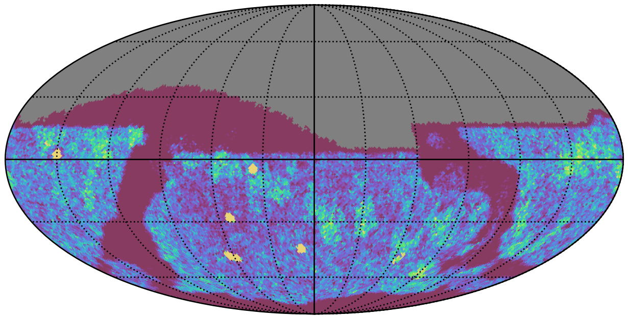
roll_uniform_early_half_mjdp67_v3.4_10yrs Yr 1 z band: NVisits
