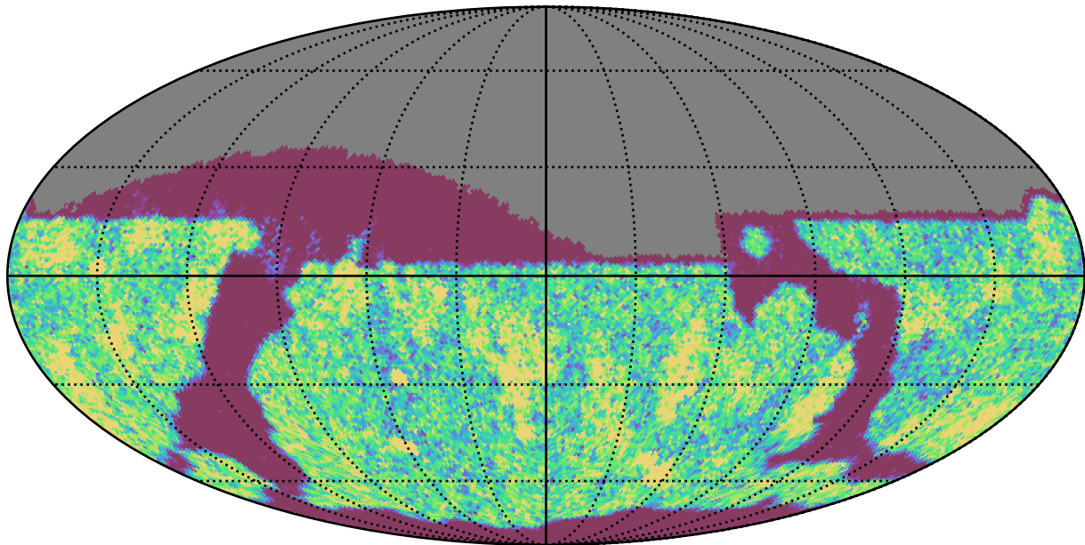
roll_uniform_early_half_mjdp67_v3.4_10yrs Yr 1 i band: NVisits
