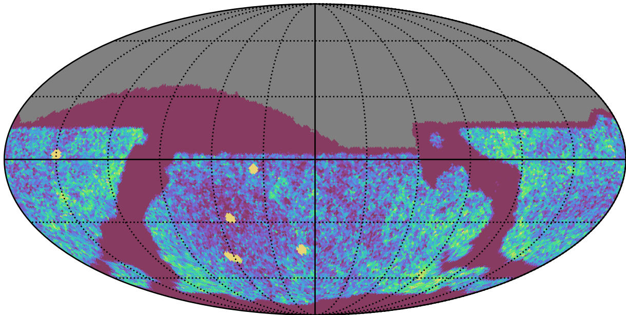
roll_uniform_early_half_mjdp67_v3.4_10yrs Yr 1 all bands: NVisits
