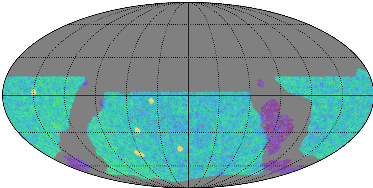
roll_uniform_early_half_mjdp67_v3.4_10yrs WFD u band: NVisits
