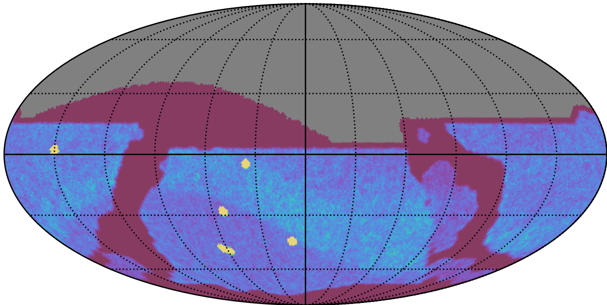
roll_uniform_early_half_mjdp67_v3.4_10yrs All sky z band: NVisits
