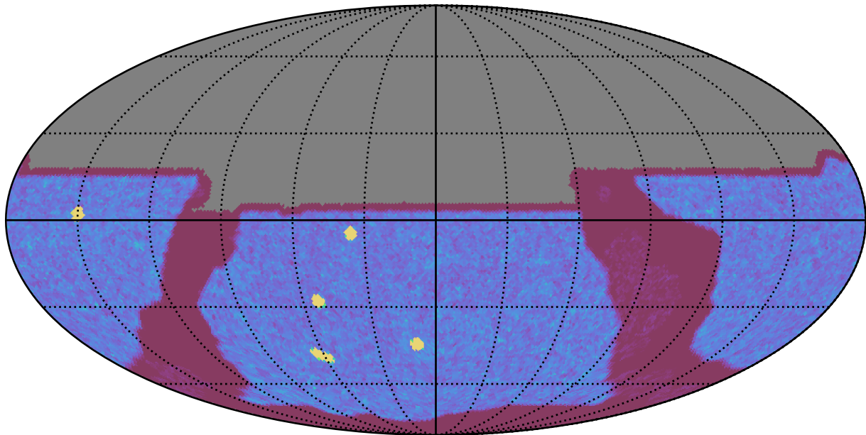
roll_uniform_early_half_mjdp67_v3.4_10yrs All sky y band: NVisits
