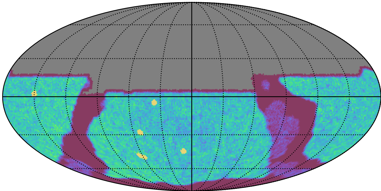
roll_uniform_early_half_mjdp67_v3.4_10yrs All sky u band: NVisits
