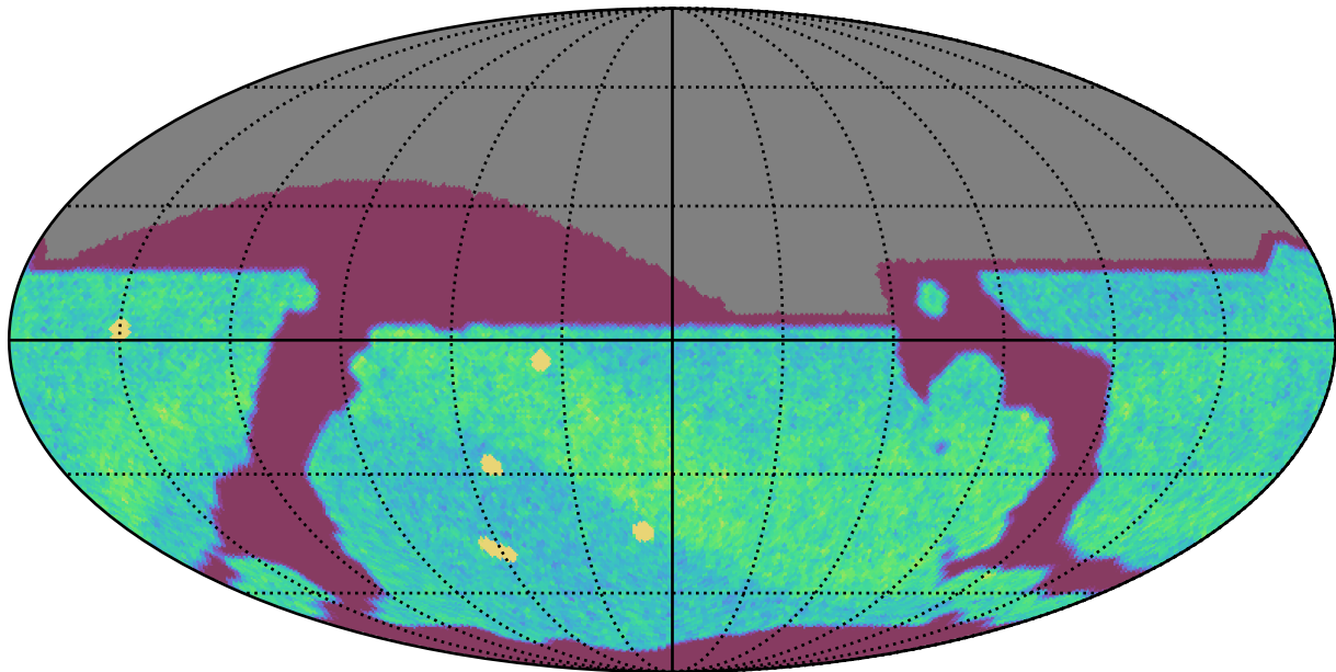
roll_uniform_early_half_mjdp67_v3.4_10yrs All sky i band: NVisits
