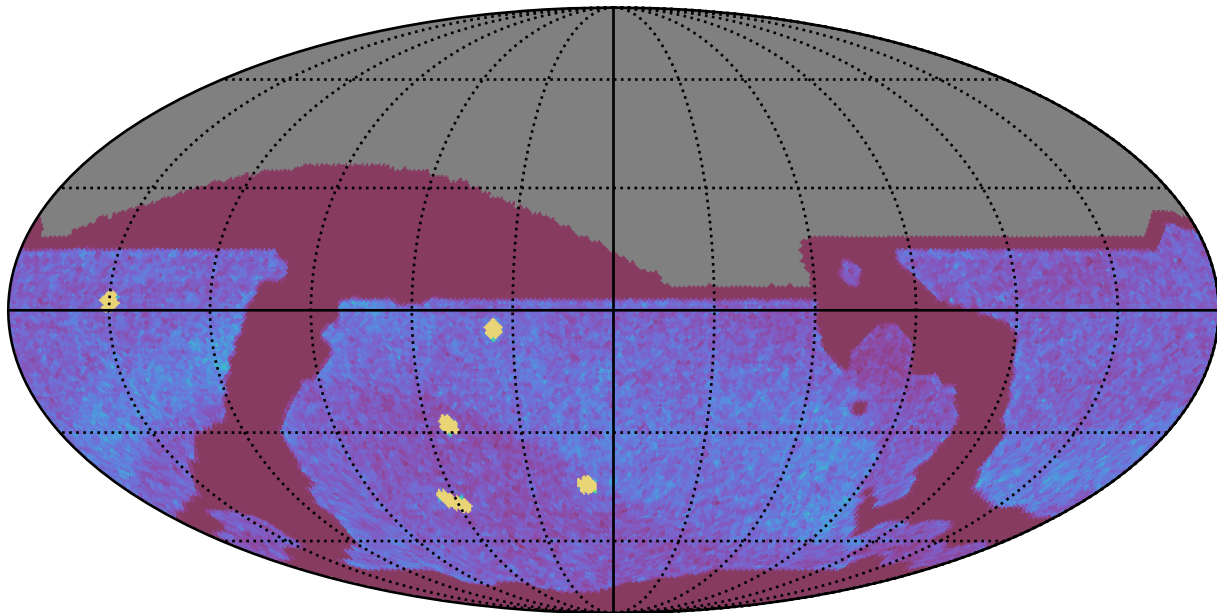
roll_uniform_early_half_mjdp67_v3.4_10yrs All sky all bands: NVisits
