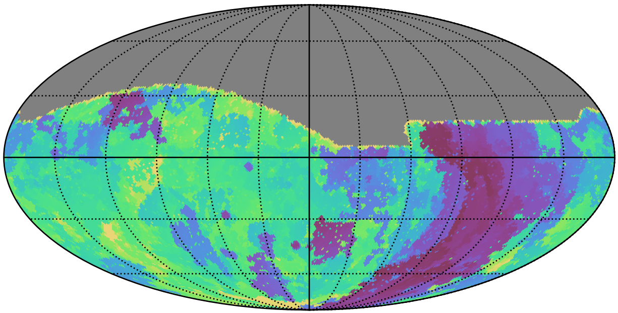
roll_uniform_early_half_mjdp67_v3.4_10yrs All sky g band: Min skyBrightness
