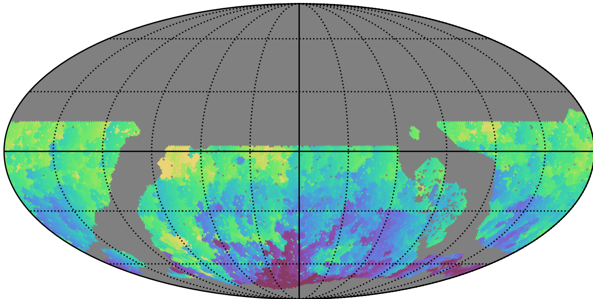
roll_uniform_early_half_mjdp67_v3.4_10yrs WFD u band: Min HA
