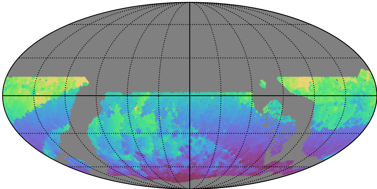
roll_uniform_early_half_mjdp67_v3.4_10yrs WFD r band: Min HA
