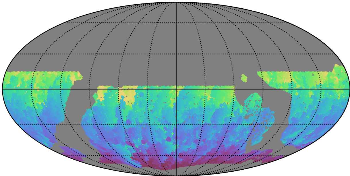
roll_uniform_early_half_mjdp67_v3.4_10yrs WFD g band: Min HA
