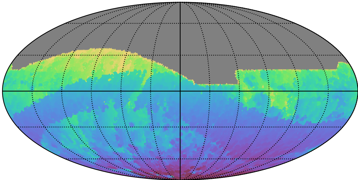
roll_uniform_early_half_mjdp67_v3.4_10yrs All sky r band: Min HA
