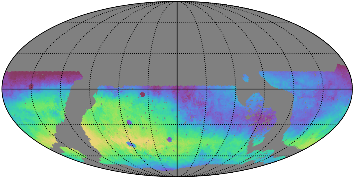
roll_uniform_early_half_mjdp67_v3.4_10yrs WFD r band: Median skyBrightness
