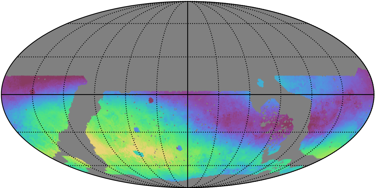
roll_uniform_early_half_mjdp67_v3.4_10yrs WFD g band: Median skyBrightness
