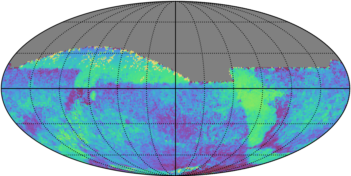
roll_uniform_early_half_mjdp67_v3.4_10yrs All sky all bands: Median skyBrightness
