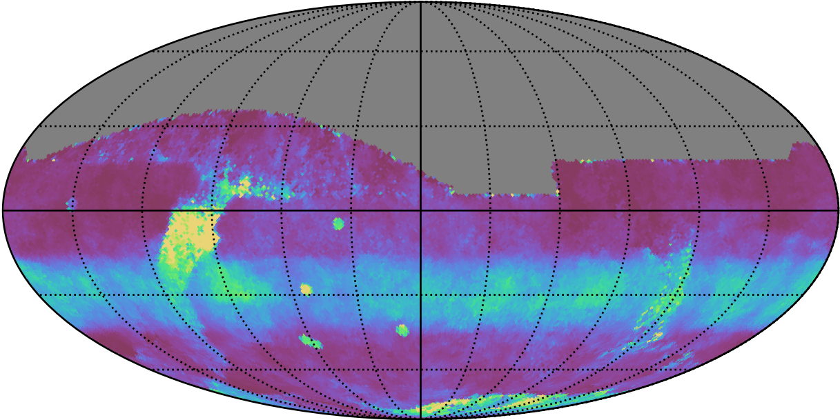
roll_uniform_early_half_mjdp67_v3.4_10yrs All sky z band: Median normairmass
