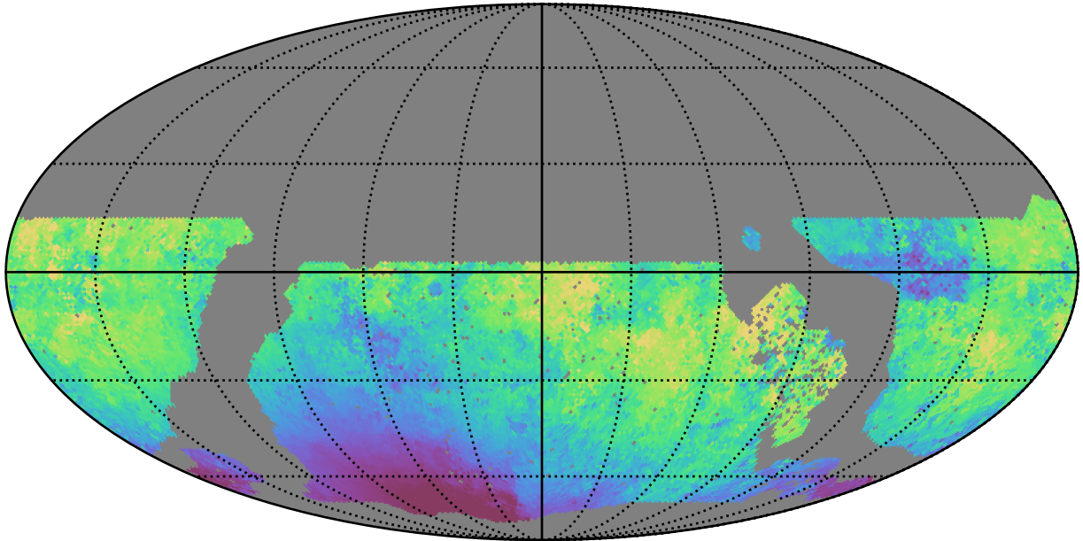
roll_uniform_early_half_mjdp67_v3.4_10yrs WFD u band: Median moonDistance
