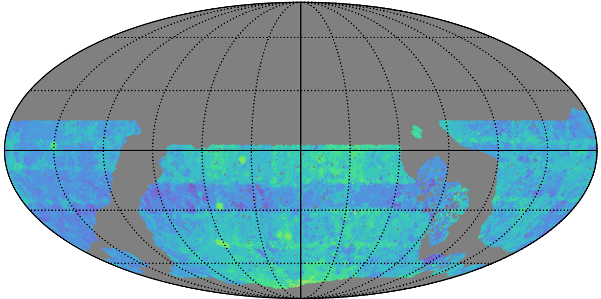
roll_uniform_early_half_mjdp67_v3.4_10yrs WFD y band: Median Season Length
