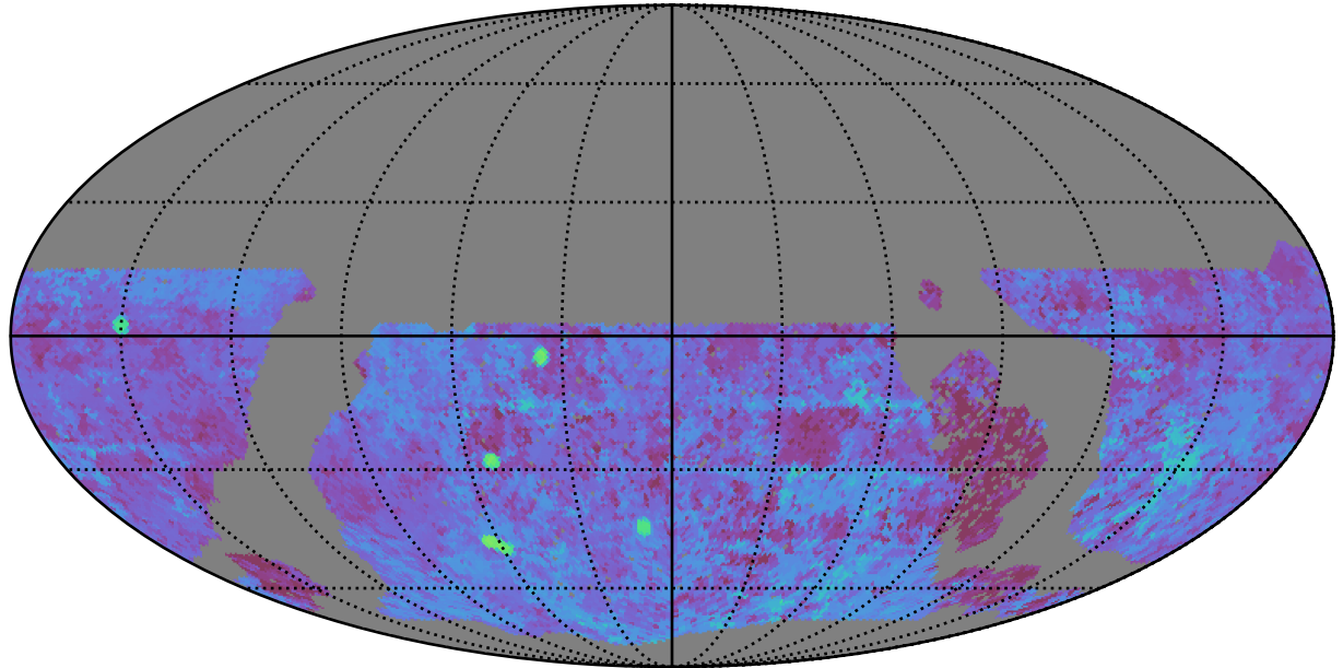
roll_uniform_early_half_mjdp67_v3.4_10yrs WFD u band: Median Season Length
