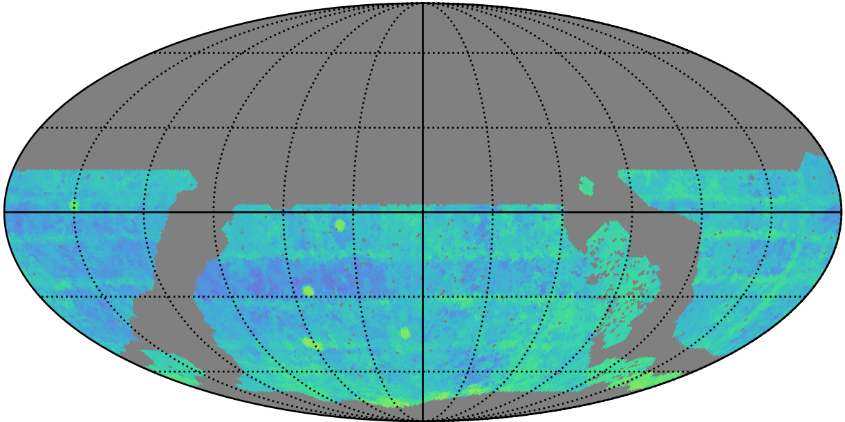
roll_uniform_early_half_mjdp67_v3.4_10yrs WFD r band: Median Season Length
