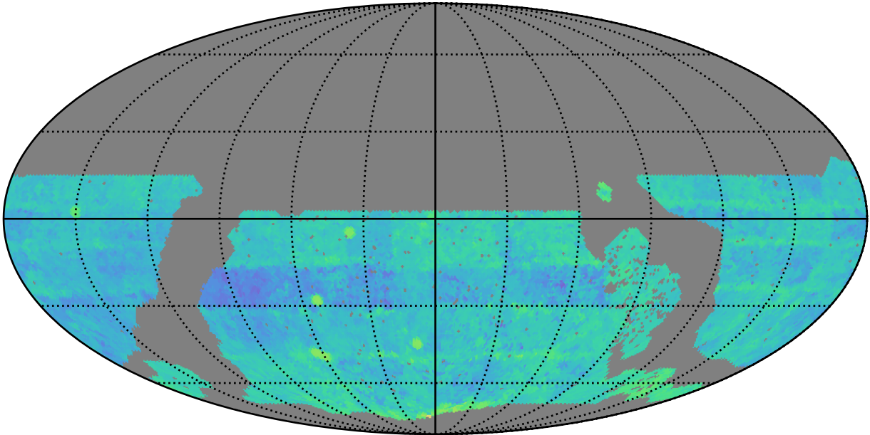
roll_uniform_early_half_mjdp67_v3.4_10yrs WFD i band: Median Season Length
