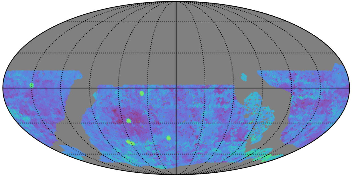
roll_uniform_early_half_mjdp67_v3.4_10yrs WFD g band: Median Season Length
