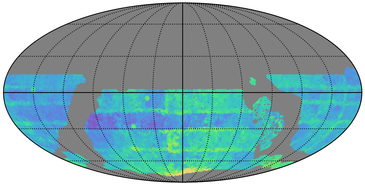
roll_uniform_early_half_mjdp67_v3.4_10yrs WFD all bands: Median Season Length
