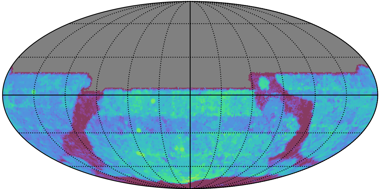
roll_uniform_early_half_mjdp67_v3.4_10yrs All sky y band: Median Season Length
