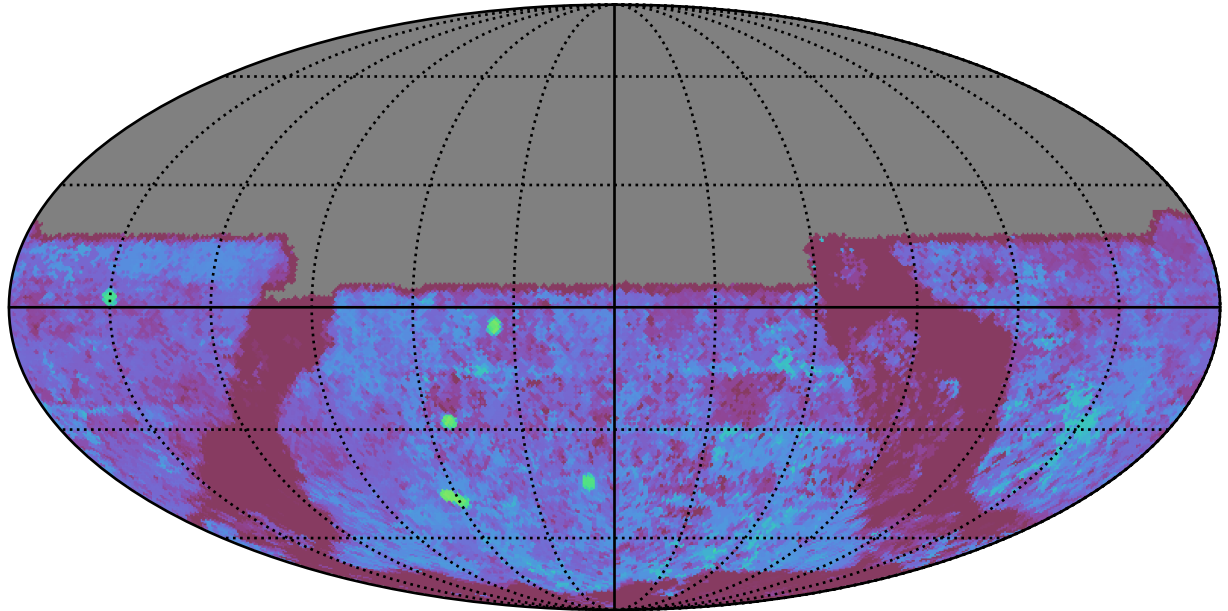
roll_uniform_early_half_mjdp67_v3.4_10yrs All sky u band: Median Season Length
