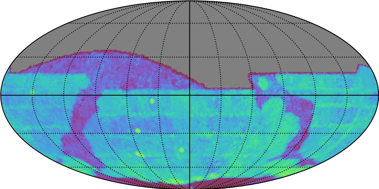
roll_uniform_early_half_mjdp67_v3.4_10yrs All sky r band: Median Season Length
