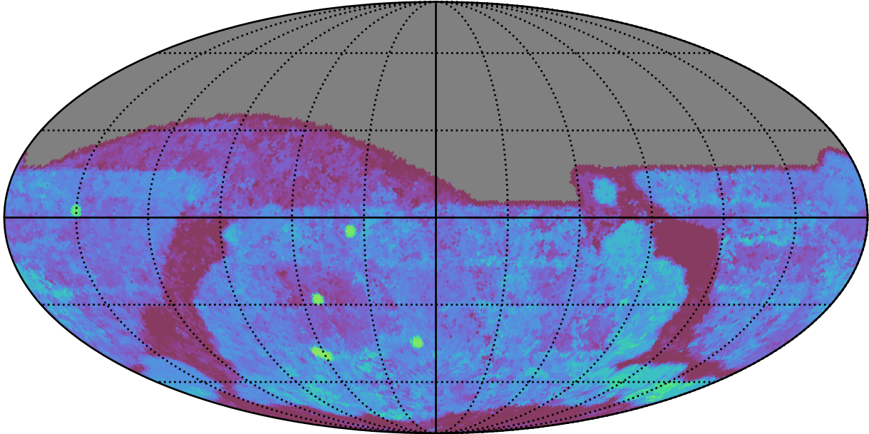
roll_uniform_early_half_mjdp67_v3.4_10yrs All sky g band: Median Season Length
