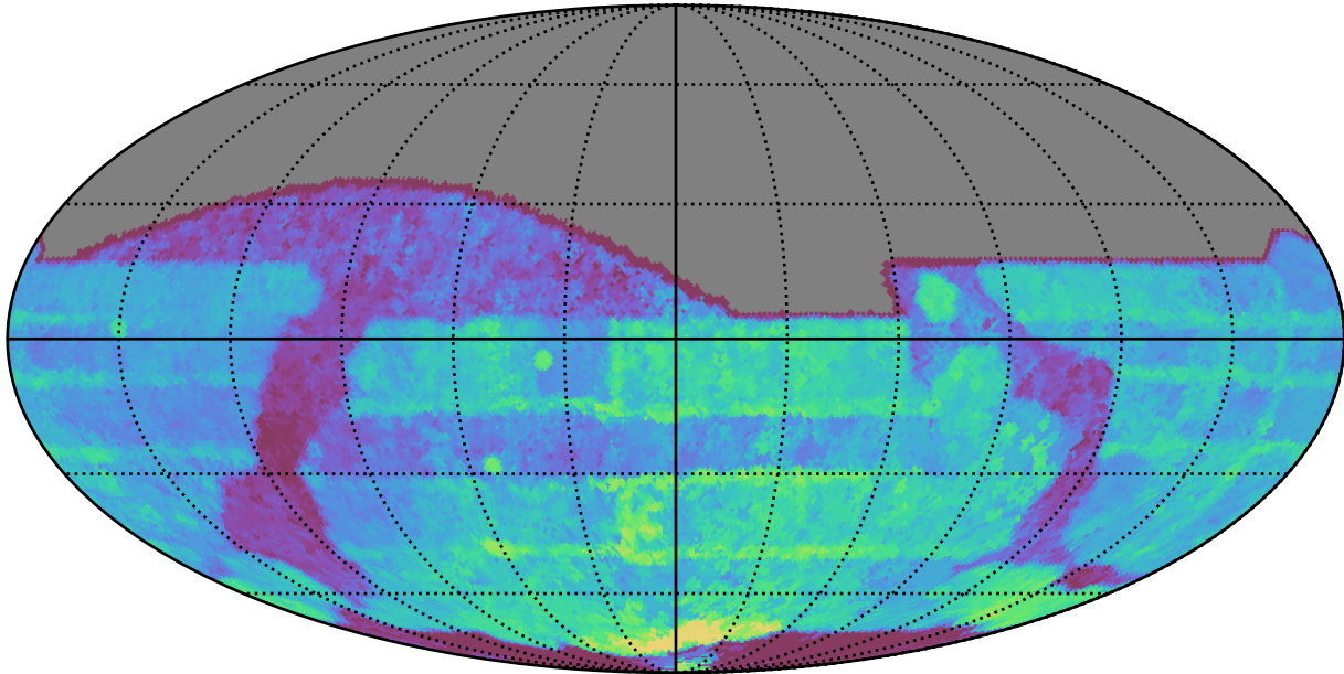
roll_uniform_early_half_mjdp67_v3.4_10yrs All sky all bands: Median Season Length
