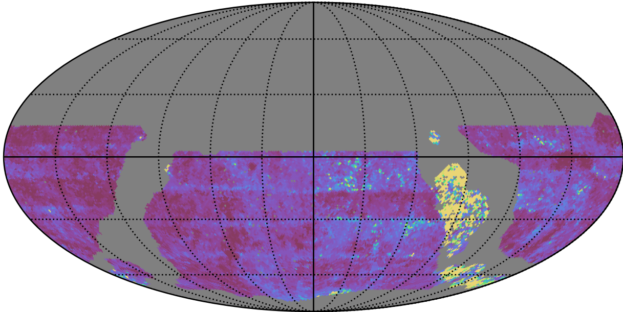
roll_uniform_early_half_mjdp67_v3.4_10yrs WFD u band: Median Inter-Night Gap
