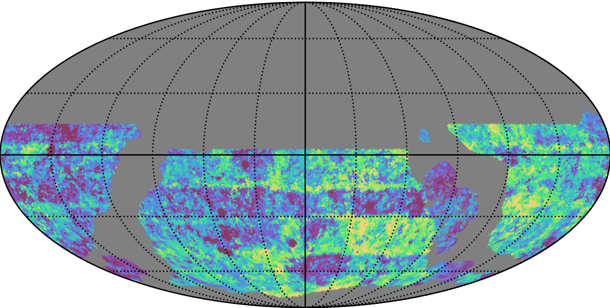
roll_uniform_early_half_mjdp67_v3.4_10yrs WFD g band: Median Inter-Night Gap
