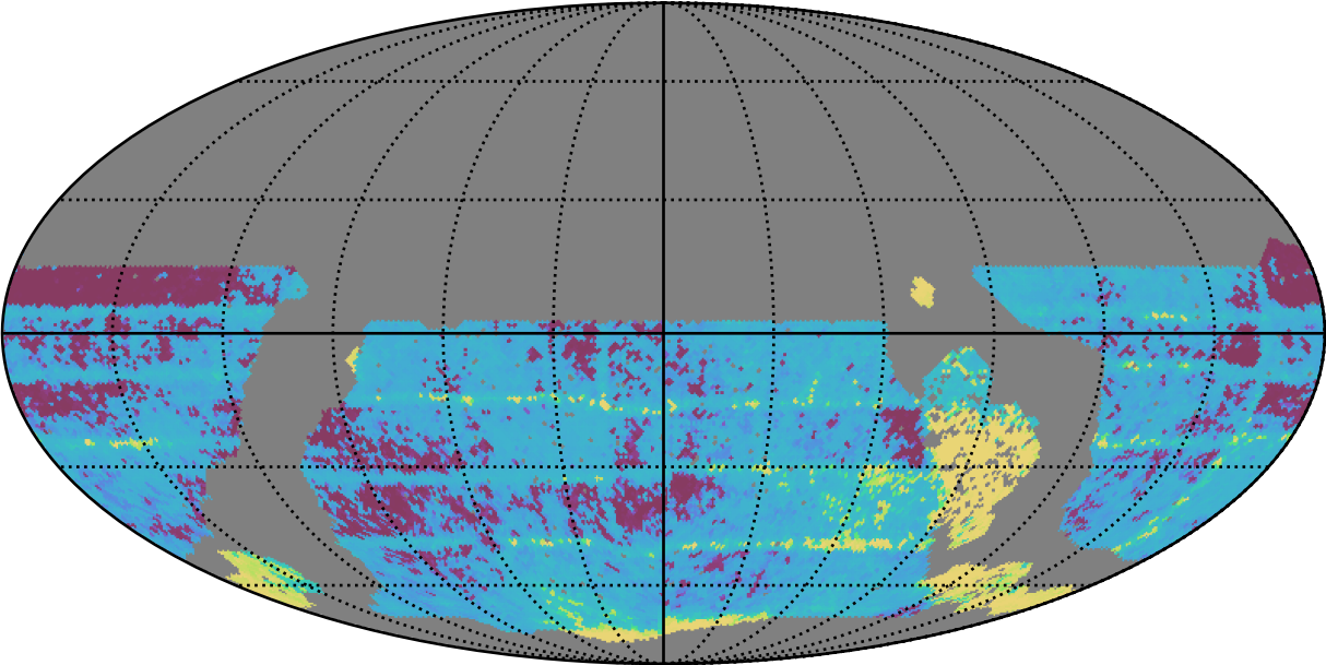
roll_uniform_early_half_mjdp67_v3.4_10yrs WFD all bands: Median Inter-Night Gap
