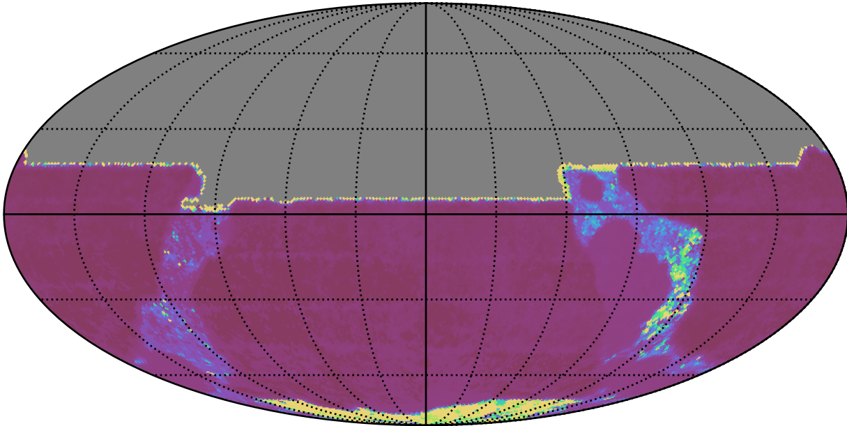
roll_uniform_early_half_mjdp67_v3.4_10yrs All sky y band: Median Inter-Night Gap
