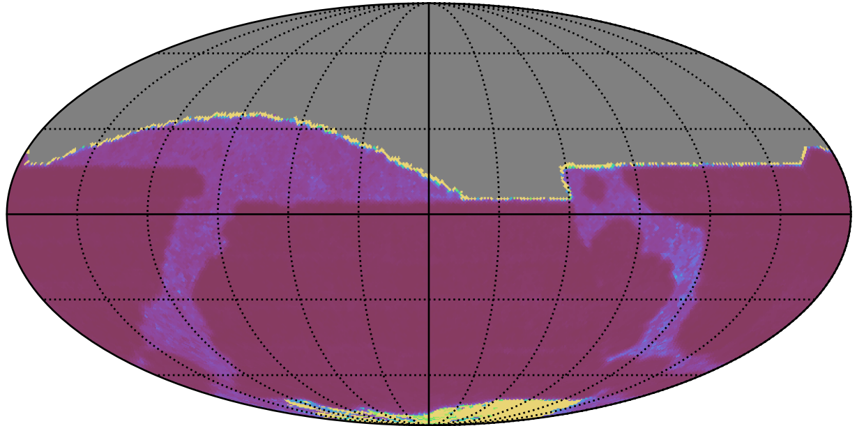
roll_uniform_early_half_mjdp67_v3.4_10yrs All sky r band: Median Inter-Night Gap
