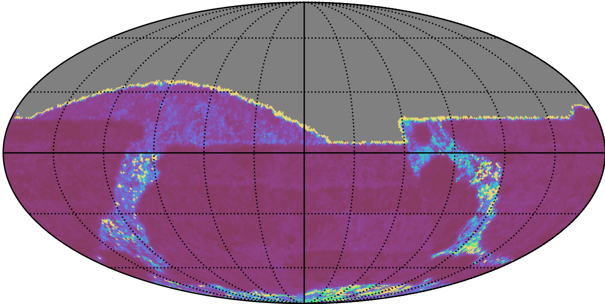
roll_uniform_early_half_mjdp67_v3.4_10yrs All sky g band: Median Inter-Night Gap
